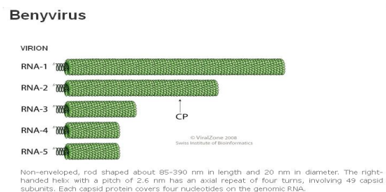
Fig. 1 Physical structure of Beny Virus
